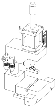
Pneumatic Press CA-120070 (supplied as shown)
