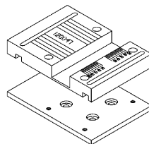
Base & Adapter Plate CA-120047 Required for use with Pneumatic press and inserts
