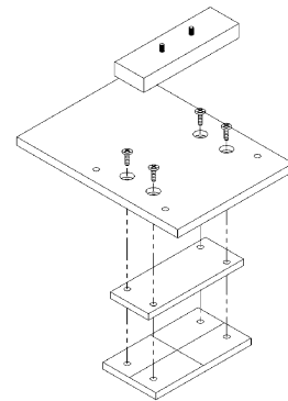
Adapter Assembly
